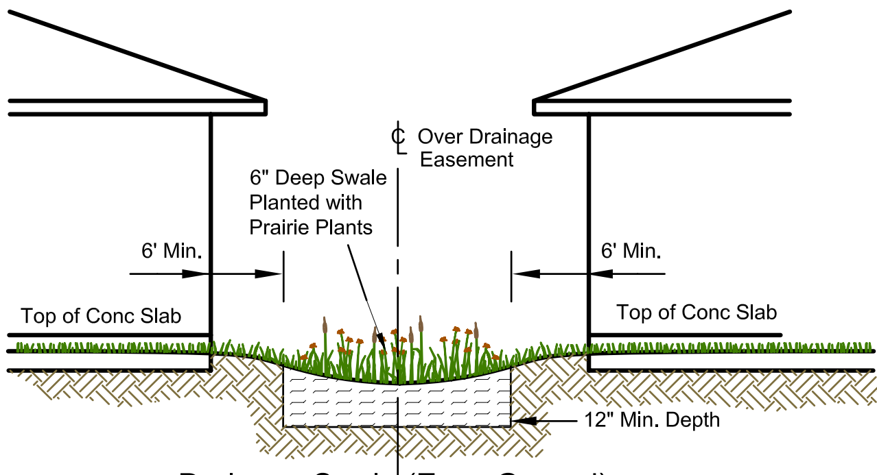
Drainage Swale (Even Ground)
