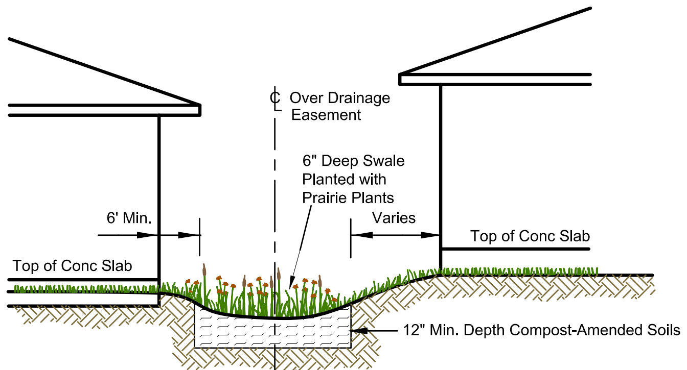
Drainage Swale (Uneven Ground)
