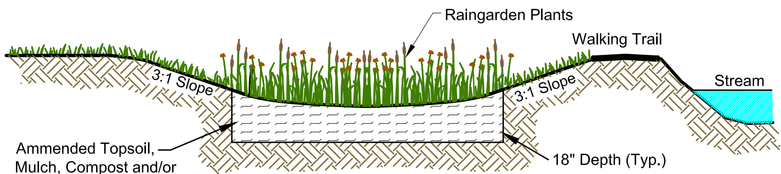
Typical Raingarden - Side View
